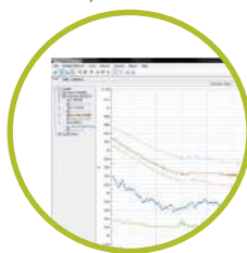
Analysis software
